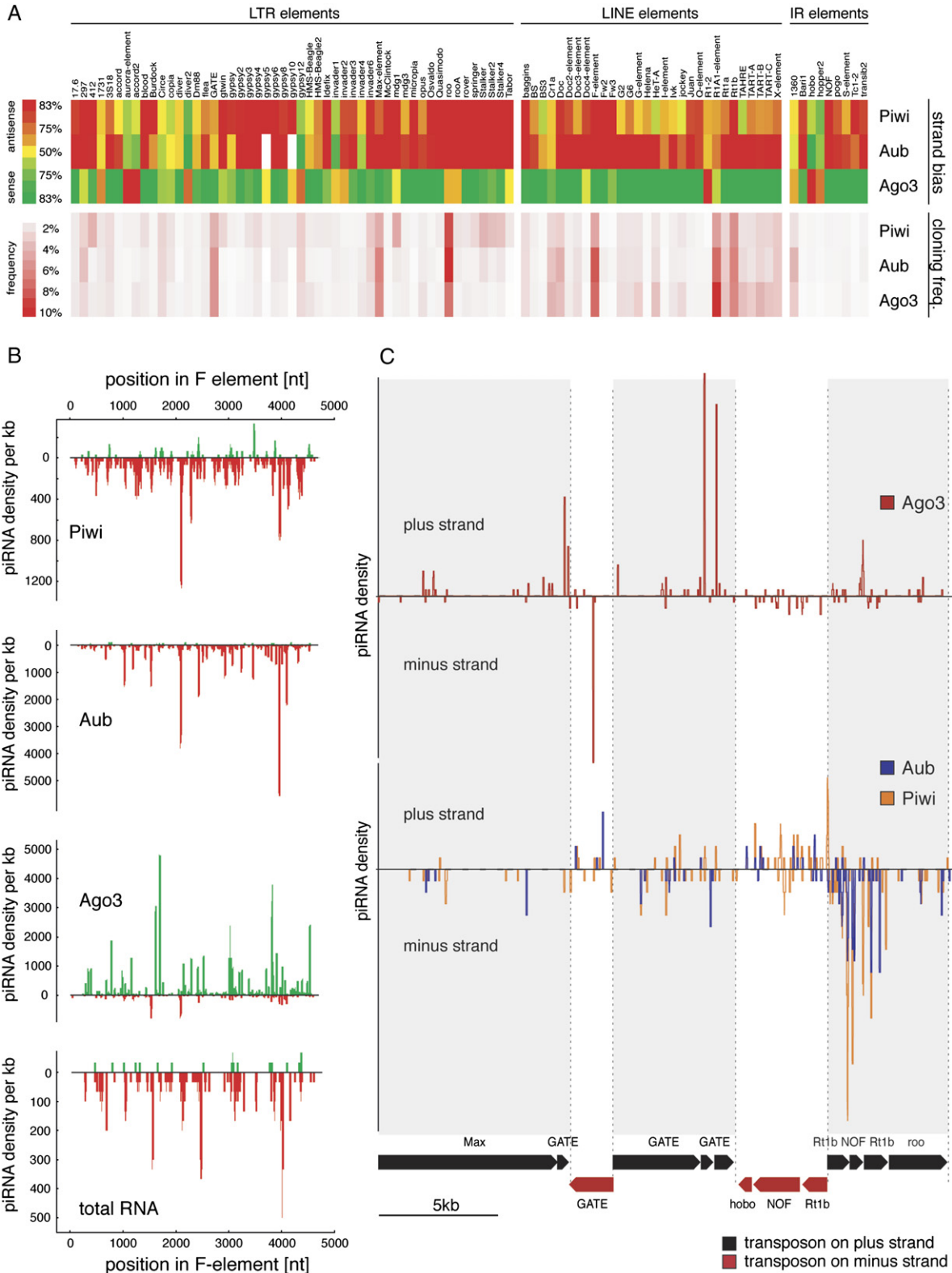
Figure 5. Piwi Complexes Show Profound Strand Biases
