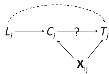
Confounder
